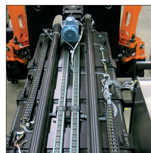
Drive unit.
